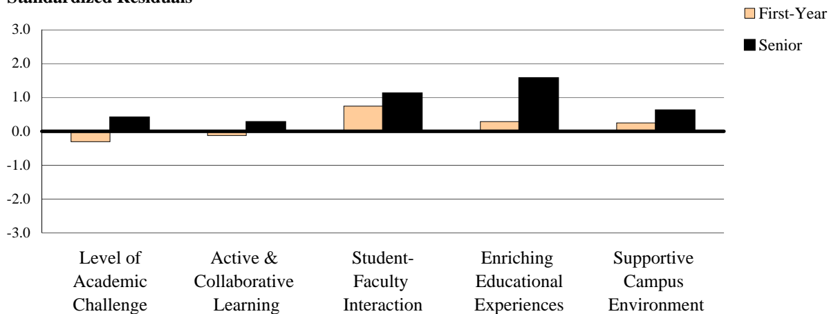
Standardized Residuals
